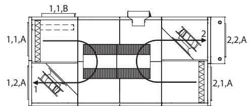
VEX370 HCWI RIGHT
