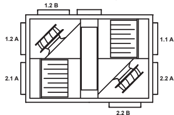
VEX200 - Posefilter Ventilatorplacering 1 - LEFT
