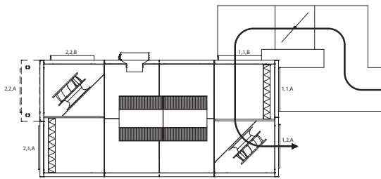
VEX370 Flue Gas LEFT
