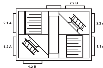
VEX200 - Posefilter Ventilatorplacering 1 - RIGHT
