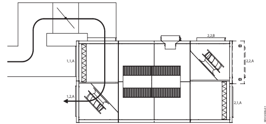
VEX370 Flue Gas RIGHT
