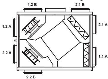
VEX100 - Horizontal/Ceiling LEFT
