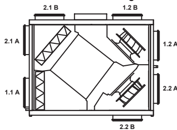
VEX100 - Horizontal/Ceiling RIGHT
