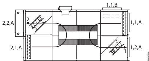
VEX370 HCWI LEFT
